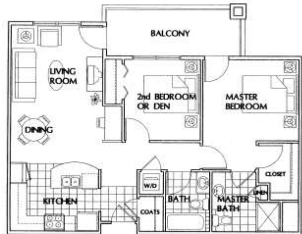
2- Bedroom Apartment 860 Sq. Ft.
